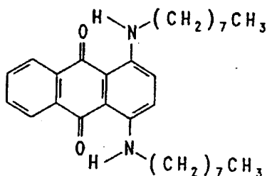
Compound 1a
